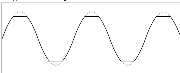
Clipped Sine Wave Signal ☹
